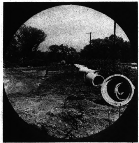
SEWER SHAPES UP — Construction on the giant Clinton-Oakland Sewer Interceptor, designed to drain six townships, gets under way in Rochester. Official ground-breaking ceremonies for the $28.2-million facility will be 10:30 a.m. Oct. 1 near the Oakland County Service Center.
