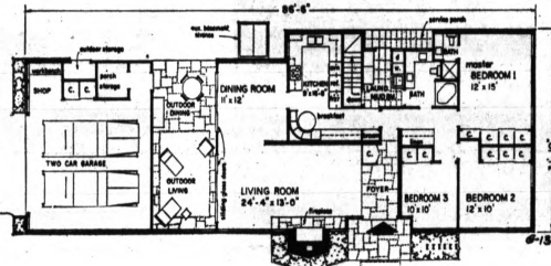
FLOOR PLAN — Excellent circulation pattern of this three-bedroom, one-story contemporary is enhanced by location of indoor-outdoor area between the basic house and the garage, making it practical extension of living room and dining room.
