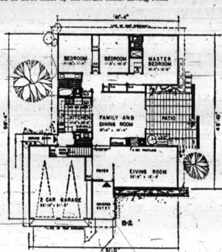
FLOOR PLAN —There are 2½ baths in this three-bedroom ranch. Modern kitchen is in central location with easy access to the outside and basement. Living area is 1,672 square feet, not including two-car garage.
