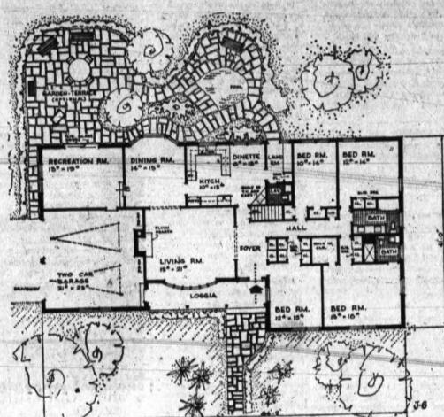
FLOOR PLAN — Straightforward plan clearly defines all living areas — sleeping, housekeeping and recreation — and the way they are related. Dimensions are 41'2" wide by 61' deep. If desired, garage doors could be located on front rather than side of house.
