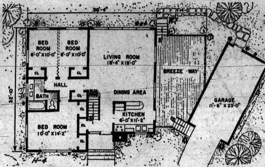
FLOOR PLAN —The basic area of this house is a modest 1,100 square feet. Optional wall divides the two family bedrooms, or else designates one of the rooms as a den. Basement is located beneath the entire living area of the house.
