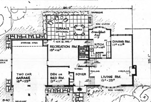
FLOOR PLANS — Grade level entrance permits routine traffic to reach kitchen without entering living room. On the upper floor, note the option which can provide a second full bath.
