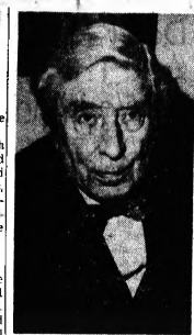
Dr. William F. G. Swann, internationally known physicist, teacher, philosopher and authority on cosmic radiation, died Monday at Swarthmore, Pa.
