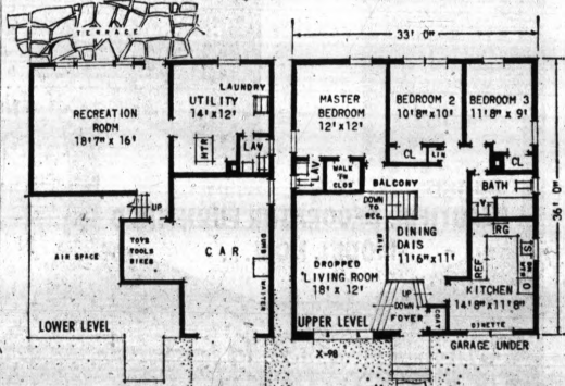
FLOOR PLAN — Unusual foyer arrangement, dining dias and living room dropped four feet below main living level provide dramatic distinction. On lower level, recreation room is the only finished space.
