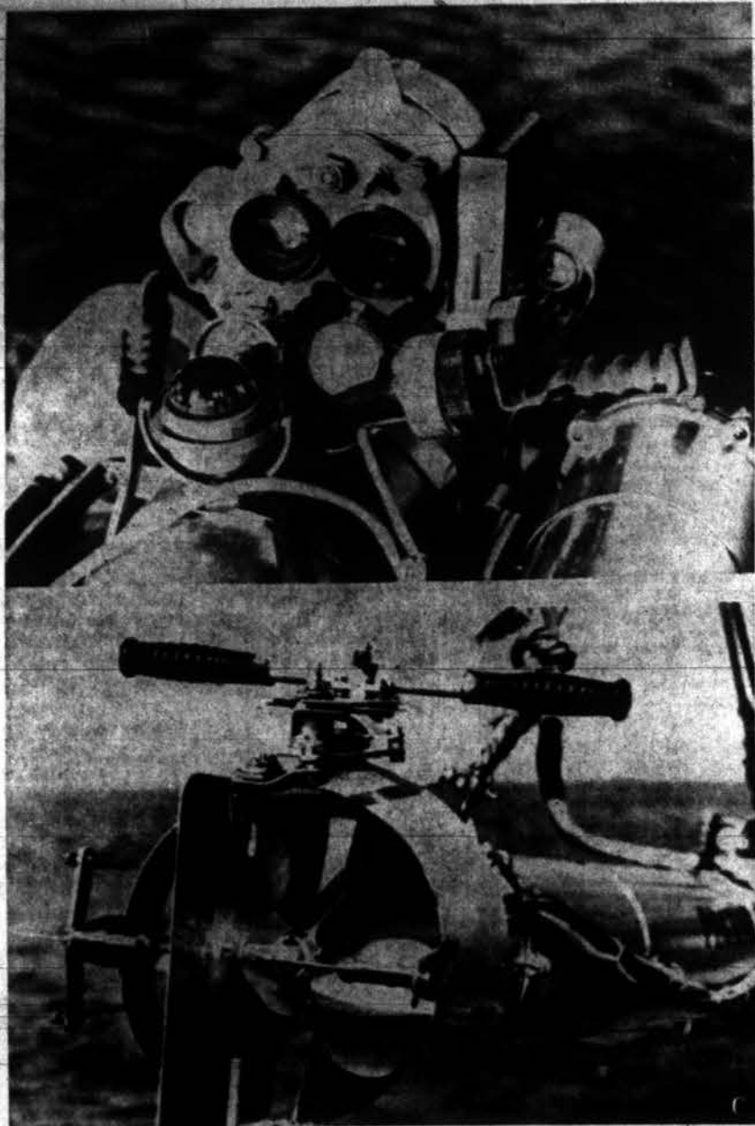
UNDERWATER EXPLORER — A new underwater vehicle, seen here from the front (top) and back (bottom), will be used next spring to photograph the sunken liner Andrea Doria. The torpedo-like device, which the diver will ride "piggyback," was developed by the Submarine
