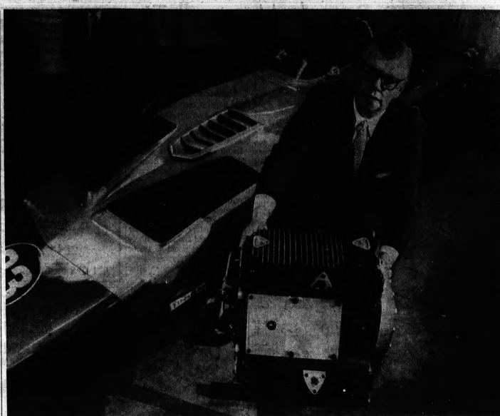
HEAD OF STEAM — William P. Lear, inventor and builder of Lear Jet aircraft, displays a steam-powered race car and the reciprocating steam engine he intends to prepare for championship class racing. The 600 horsepower engine
