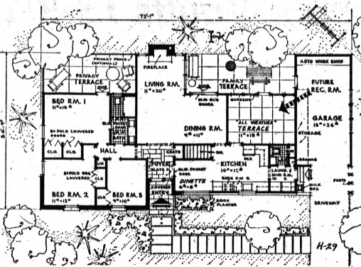
FLOOR PLAN—Center hall arrangement assures good circulation in this well-designed home. The all-weather terrace can be walled on the fourth side as a future recreation room, and the family terrace screened.
