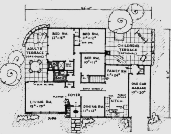
FLOOR PLAN — Center hall splits the T-shape of this departure from usual ranch design. Note excellent isolation of living room.
