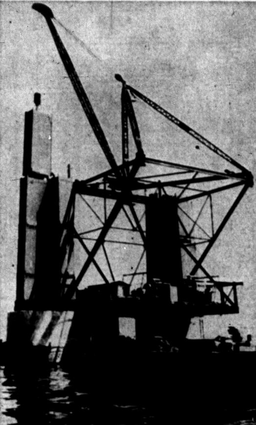
REACHING FOR THE SKY — The legs of the north main tower of the $100 million Mackinac Bridge rise to skyscraper heights as American Bridge Division briggers place the first section of the fourth tier. Shown in action here is the unique 'Crepper' derrick which raises itself between the tower legs as additional sections of the tower are added. The towers this week approach the half way mark of their eventual full height of 552 feet.
