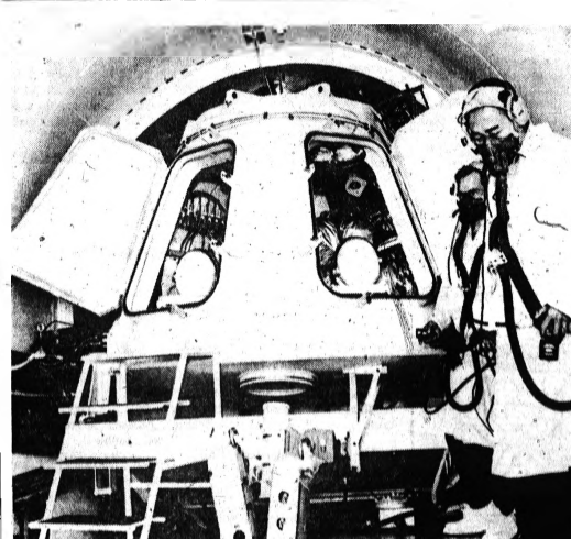
AP Photos SPACECRAFT TESTED — Space, suited engineers Bert North and Karl F. Jackson are pictured inside a Gemini space capsule in Los Angeles yesterday after two hours at simulated orbital altitude. It was the first public demonstration of an improved environmental control system to be used in the two-man capsules. The technicians at right wear oxygen masks because they had to work inside a pressure chamber during the test.
