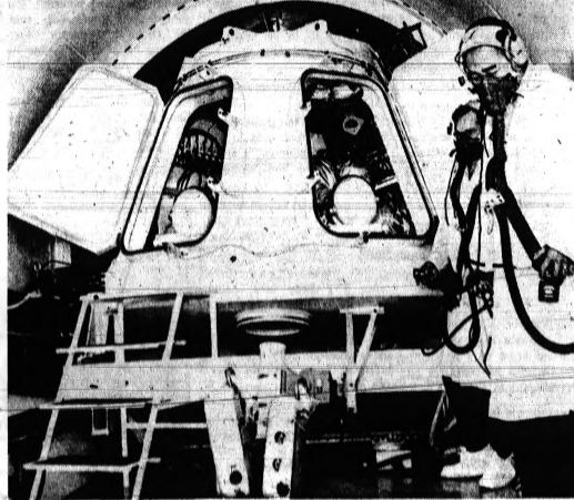
SPACECRAFT TESTED — Space-suited engineers Bert North and Karl F. Jackson are pictured inside a Gemini space capsule in Los Angeles yesterday after two hours at simulated orbital altitude. It was the first public demonstration of an improved environmental control system to be used in the two-man capsules. The technicians at right wear oxygen masks because they had to work inside a pressure chamber during the test.
