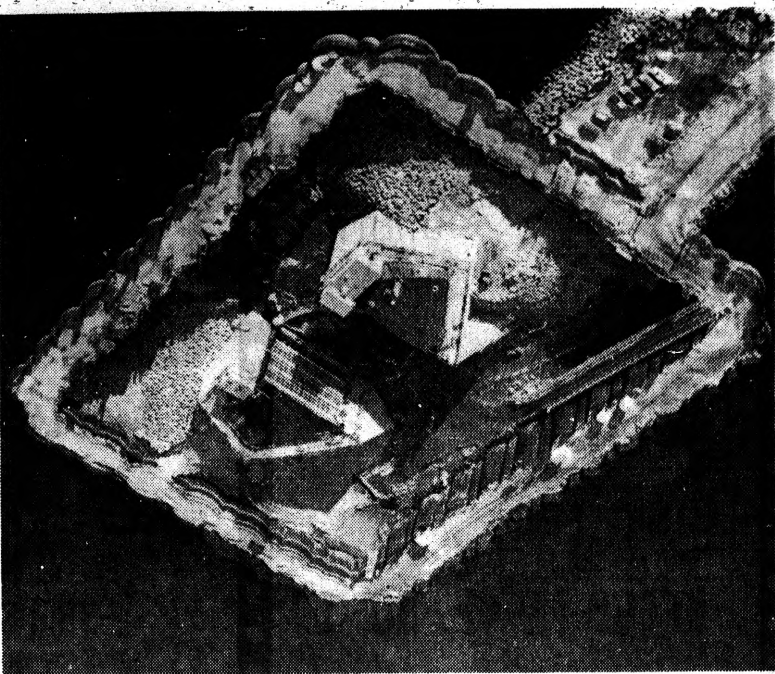
$4-MILLION HOLE —This is an air view of 400 by 650-foot cofferdam surrounding massive gates under construction for $18-million hurricane barrier at New Bedford, Mass. The gates in mile-long dike will be on either side of 150-foot ship channel and can be closed when hurricane threatens this old whaling port now a busy fishing center. This part of barrier cost $4 million.
