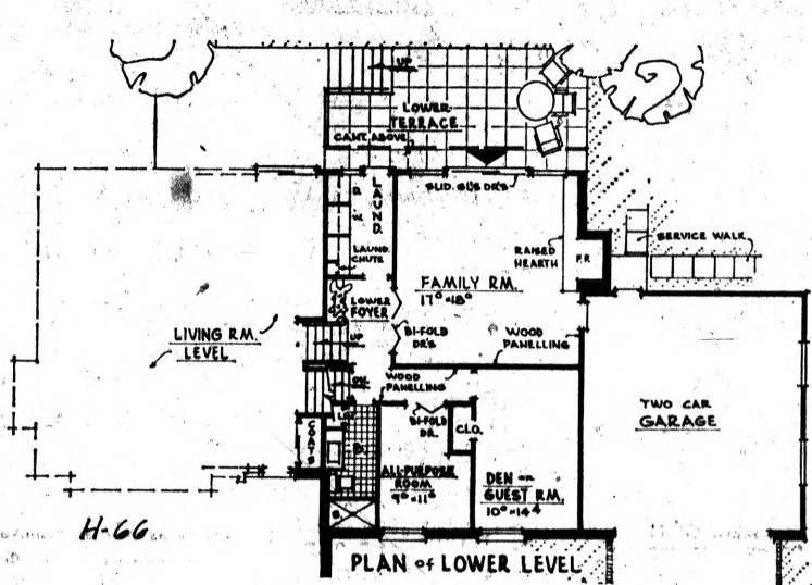
FLOOR PLANS: The three levels of Design H-66 provide lots of living space for a big family, with 1686 square feet of habitable area on the upper levels and 818 square feet on the lower level, excluding the covered entry.
