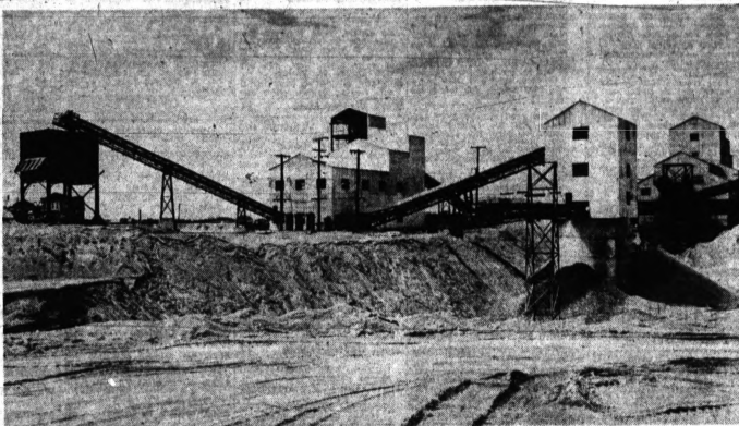
HEAVY MEDIA PLANT — The building furthest east from the road at American Aggregates, north of Oxford, houses a giant drum that separates deleterious stones from 'AA' gravel by a "heavy media" process that floats away the lighter-weight
