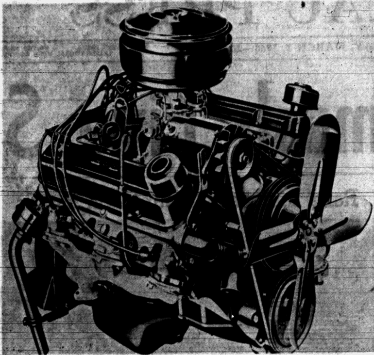
BLUE CHIP V-8 — The 180-horsepower rating of GMC's new engine tops last year's by 25 horsepower and is the biggest short-stroke V-8 in its field. With a 316 cubic inch displacement, the engine is available in every basic model in the light and medium duty class (100-370 series). Story on page one.
