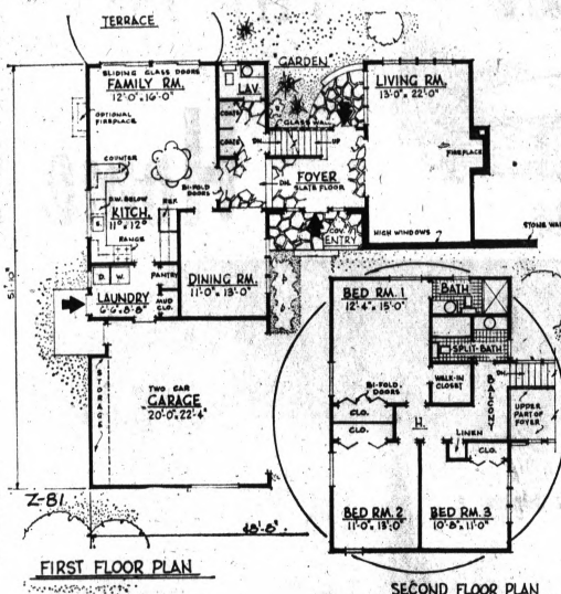
FLOOR PLANS — Different but practical floor arrangement keeps living room for formal entertaining while permitting the family room-kitchen, with a combined length of 24', to be used for informal living for members of the family as well as guests.
