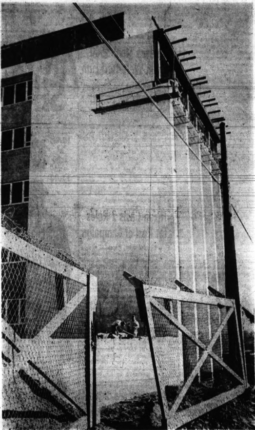
NORTHWEST CORNER — Workmen in the foreground demonstrate the size of Oakland County's new courthouse. The scaffolding near the top of the six-story structure is for the workmen adding slab after slab of the white Georgia marble facing.
