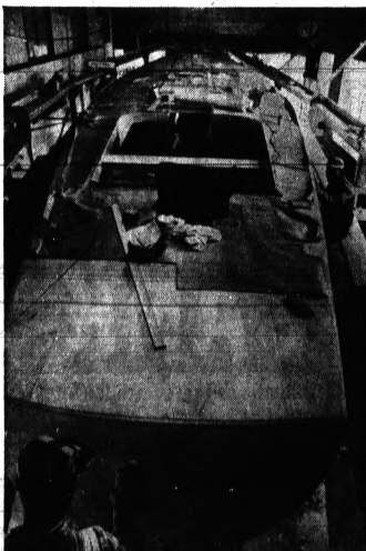
Constellation's hull takes shape at Minneford's City Island yard. It too will boast design innovations.
