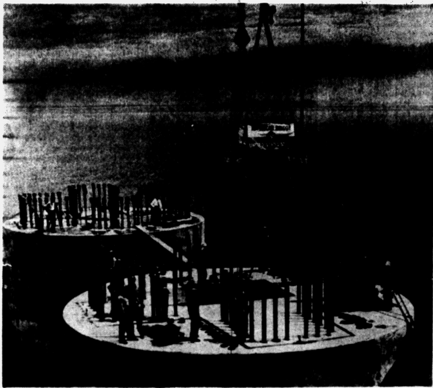
13-TON BASE PLATE FOR TOWER — This 13-ton base plate section is lowered into place on tower foundation in preparation for erection of first vertical steel on $100,000,000 Mackinac Bridge, which will be world's longest suspension span when completed in November, 1957. Tower to be built on top of base plates will be 552 feet high.
