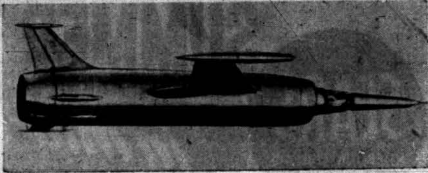
"FLYING STOVEPIPE"—This is the first photo released by the French Air Ministry showing the new supersonic Leduc 022, being tested at France's Istres airfield. The odd-looking aircraft, dubbed "The Flying Stovepipe," is powered by a ramjet engine that develops 600,000 horsepower. The eight-ton plane, made of heat-resistant alloys, is reported capable of flying at twice the speed of sound. The pilot flies in a prone position in its nose.
