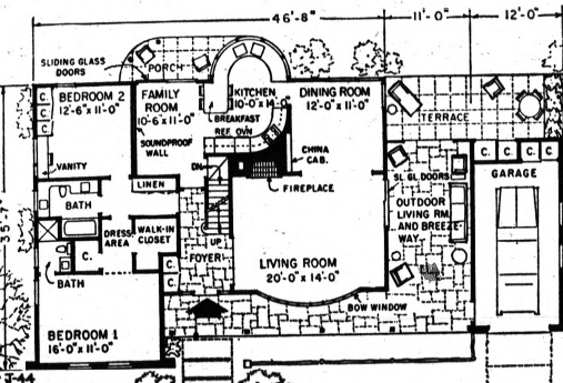
FLOOR PLANS — Living area of house contains 1,413 square feet on main floor not counting garage and porches. Expansion second floor contains 833 square feet. Unusual
