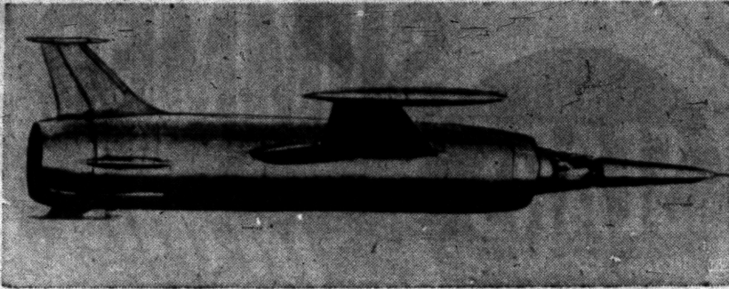
"FLYING STOVEPIPE" — This is the first photo released by the French Air Ministry showing the new supersonic Leduc 022, being tested at France's Istres airfield. The odd-looking aircraft, dubbed "The Flying Stovepipe," is powered by a ramjet engine that develops 600,000 horsepower. The eight-ton plane, made of heat-resistant alloys, is reported capable of flying at twice the speed of sound. The pilot flies in a prone position in its nose.
